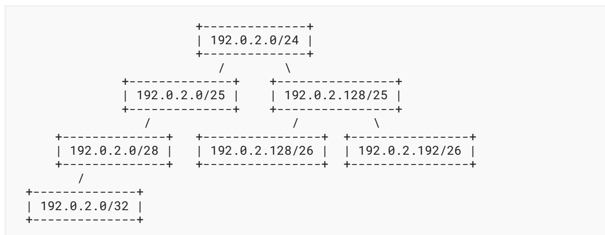
Figure 1: Example Registry Objects
